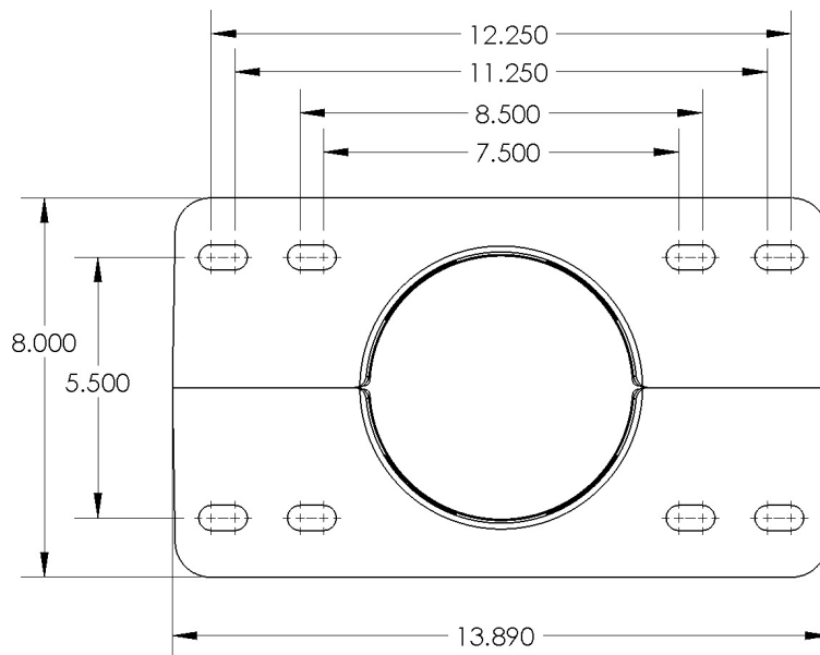
Standard Rapid Mount Mounting Pattern
