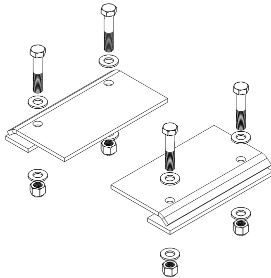
I-Beam Clamps &amp; I-Beam Bolt Kit
