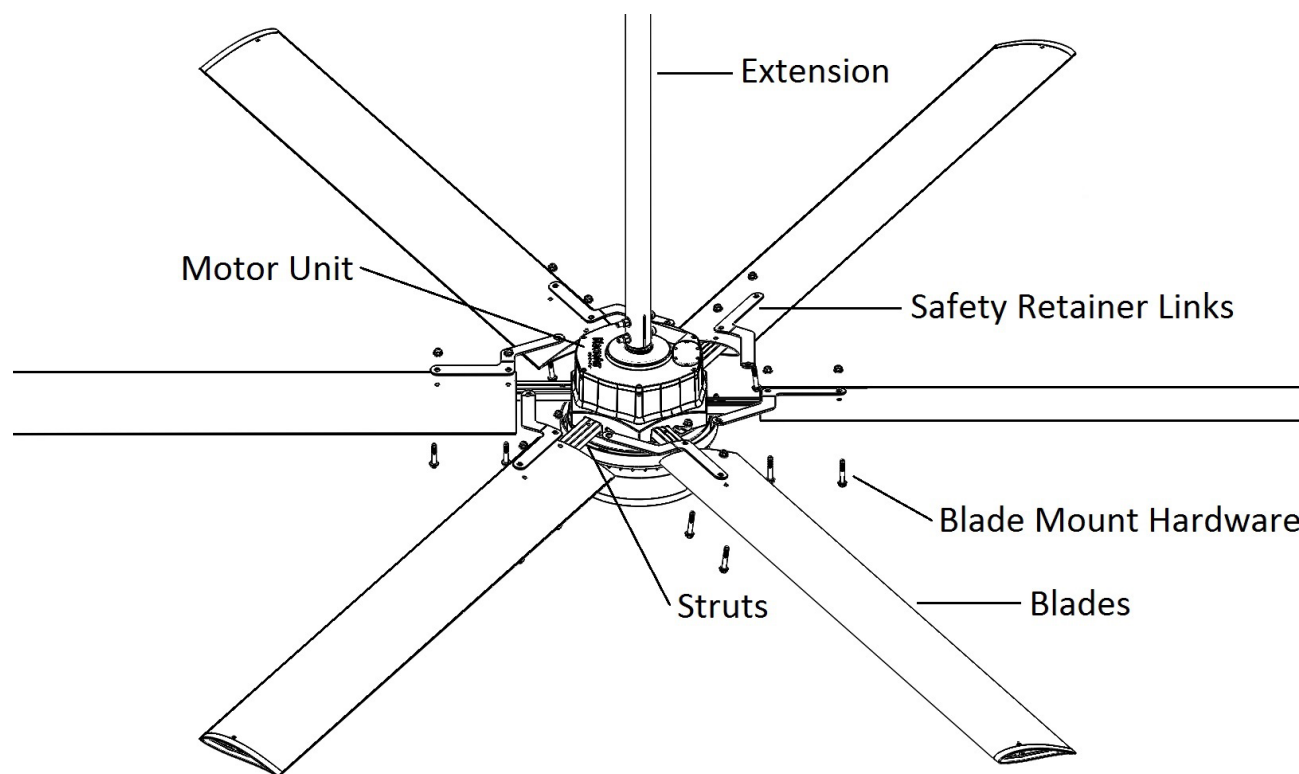
Exploded View of Fan
