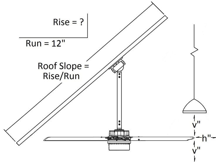
Figure 5: Fan Clearance
