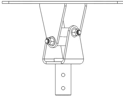
Universal Mount (standard)
