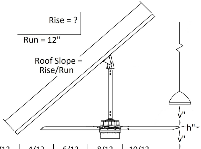
Figure 2: Fan Clearance
